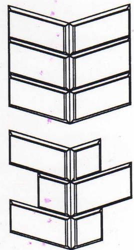
Quoin in section
